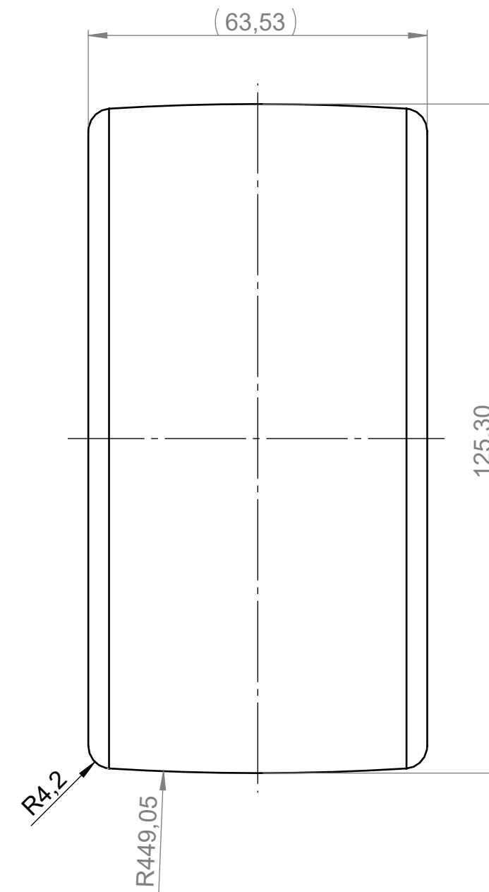
Frontscheibe Front Panel (B5503201)
