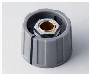
A2623068 ROUND KNOB 23, with line ABS (UL 94 HB) dusty grey RAL 7037 23x15mm 6mm
