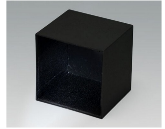
A8046408 POTTING BOXES, Vers. III PA 66 (UL 94 HB) black RAL 9005 46,2x46,2x40,8mm
