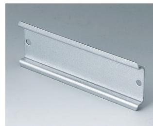
C7112077 Standard DIN rail, Type TH 35 Steel 108x35x7,5mm
