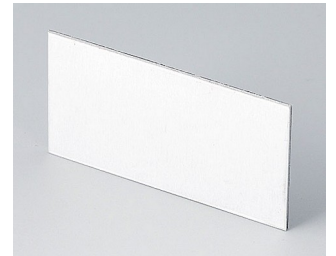
B6121112 Rear panel Aluminium matt anodised 57,6x28,6x1mm
