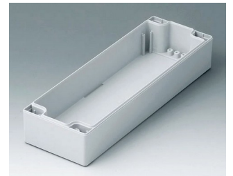
C1082402 Coquille 80, sans joint PC (UL 94 HB) gris clair RAL 7035 240x80x40mm
