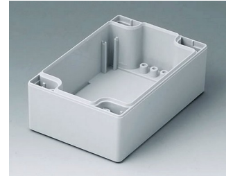
C1081202 Coquille 80, sans joint PC (UL 94 HB) gris clair RAL 7035 120x80x40mm
