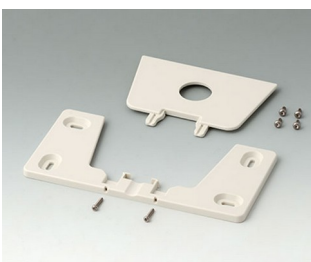
A9506117 Wall suspension element ASA+PC (UL 94 V-0) off-white RAL 9002
