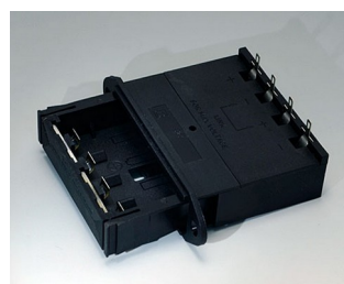
A9302540 Battery holder, 4 x AA PA (UL 94 HB) black RAL 9005
